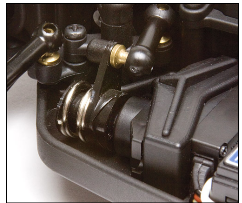
Newly designed servo saver.
